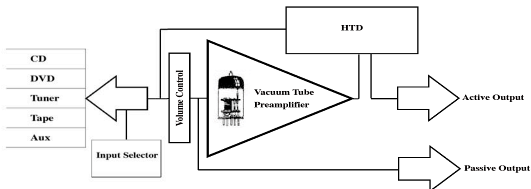
Schema a blocchi / Block Diagram
