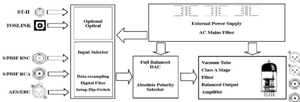
Schema a blocchi / Block Diagram
