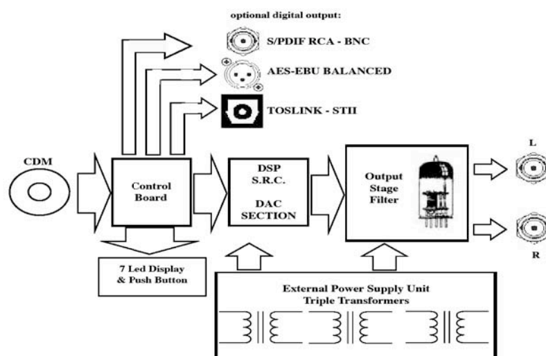
Schema a blocchi / Block Diagram
