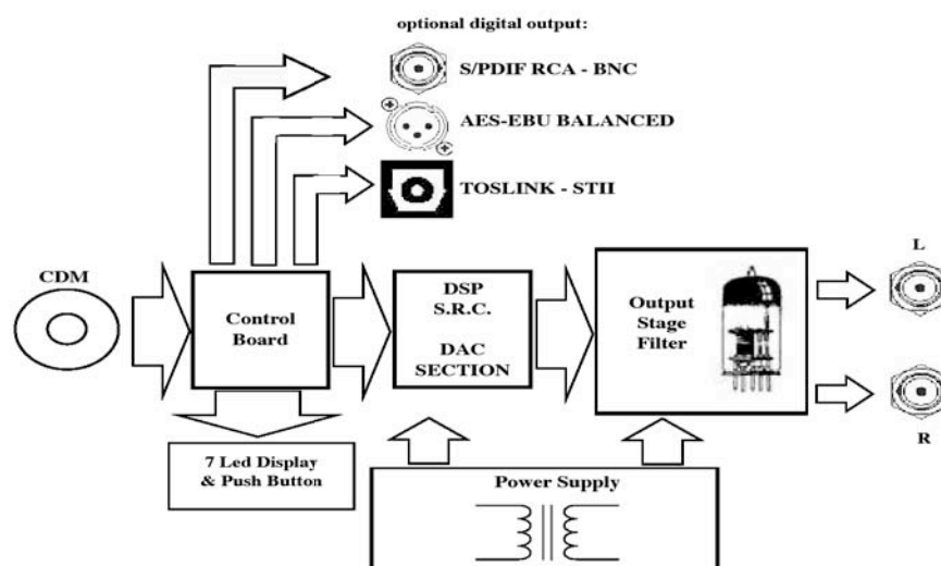
Schema a blocchi / Block Diagram
