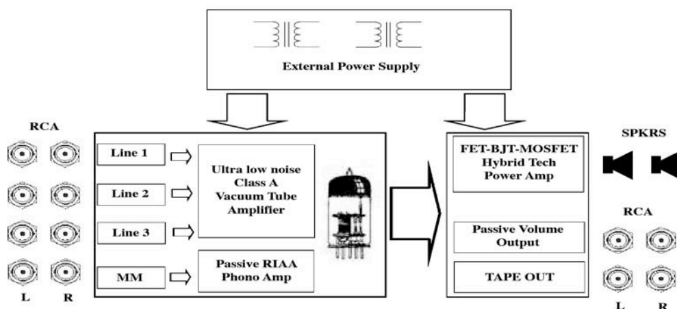
Schema a blocchi / Block Diagram
