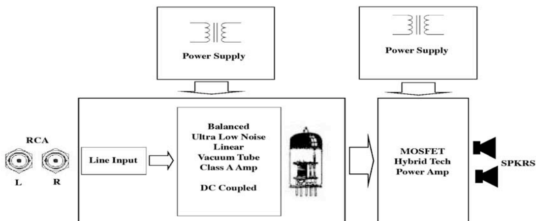
Schema a blocchi / Block Diagram
