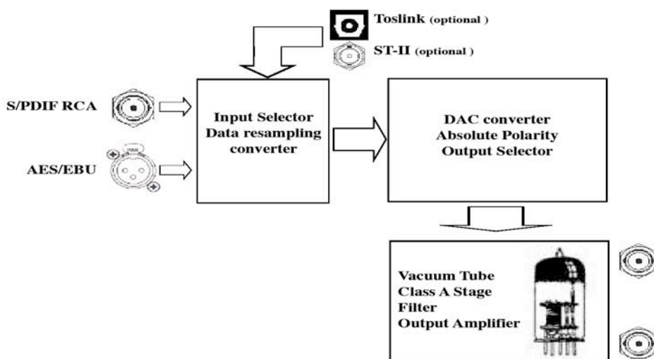
Schema a blocchi / Block Diagram
